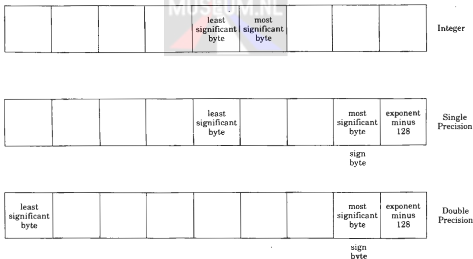
Figure D.3 Number Types in the Floating-Point Accumulator
