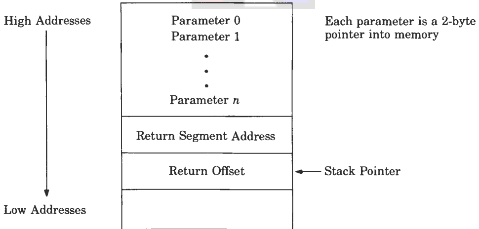
Figure D.1 Stack Layout When the CALL Statement is Activated
