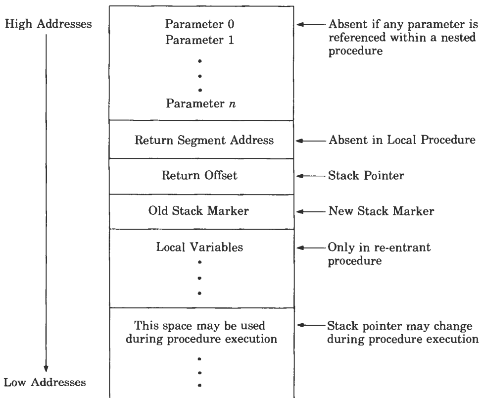
Figure D.2 Stack Layout During Execution of a CALL Statement
