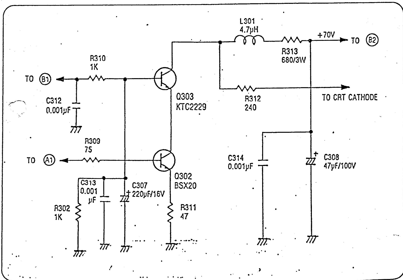
Fig. 3 Video Amplifier
